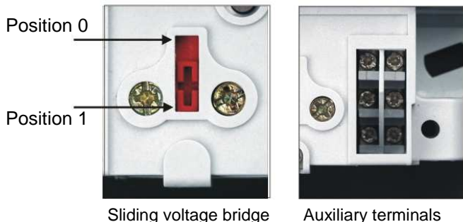
Fig. 12a: A terminal block – sliding voltage bridge and auxiliary terminals
