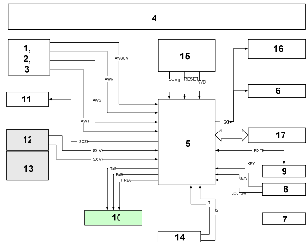
Fig. 20: MT372 meter block diagram
