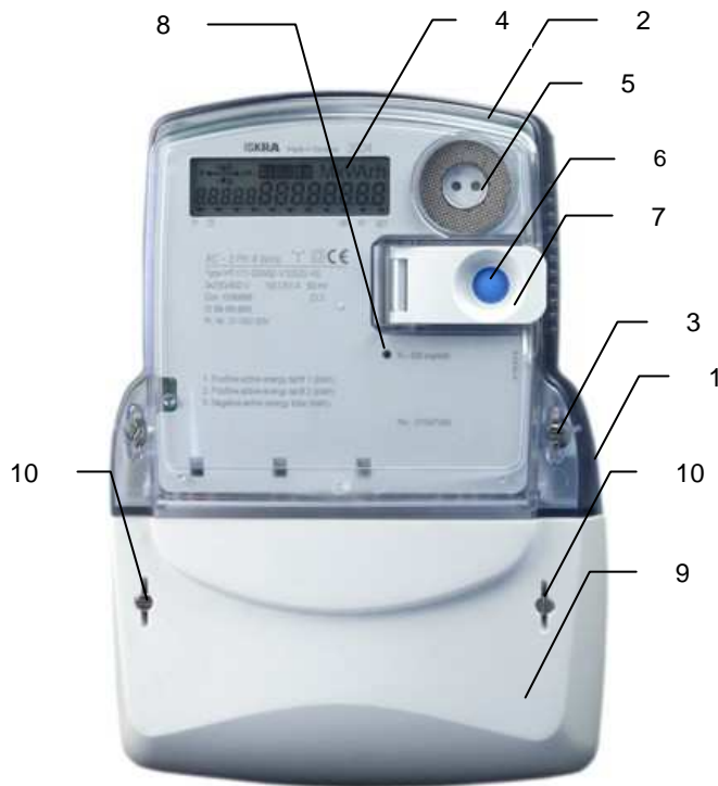
Fig. 8: MT371 meter constituent parts
