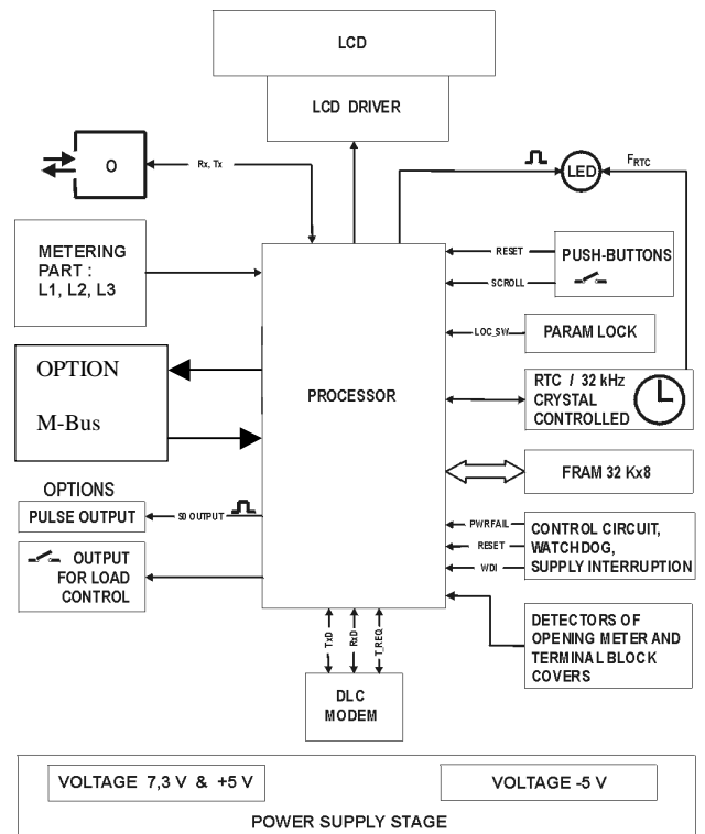
Fig. 19: MT371 meter block diagram
