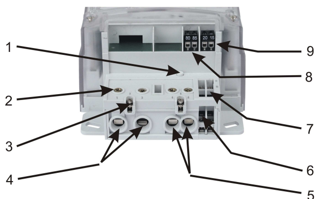
Fig. 4: A terminal block of ME37y meter
