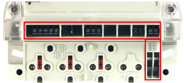
Fig. 33: Position of inputs and outputs on MT372 meter – front view
