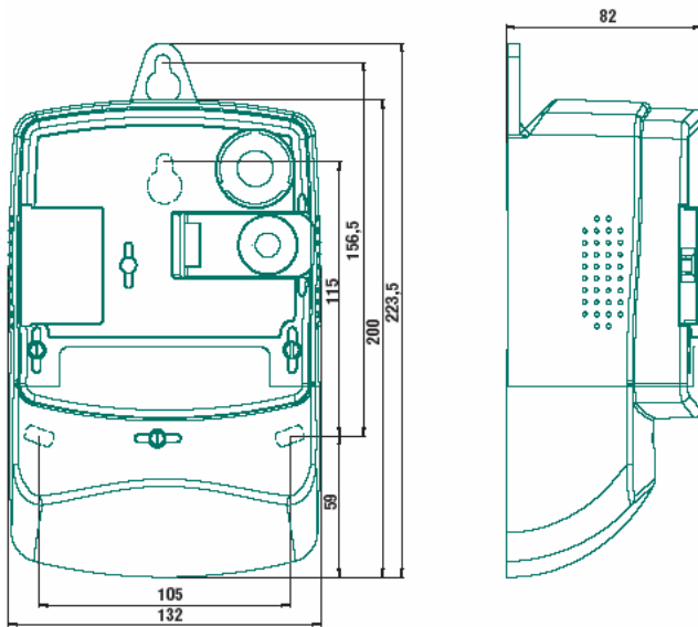
Fig. 5a: Overall and fixing dimensions of a meter fitted with a long terminal cover
