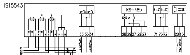
Fig. 48: Connection diagram of MT372 meter with RS 485 communication interface
