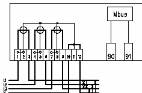
Fig. 46: Connection diagram of MT371 meter with M-Bus communication interface
