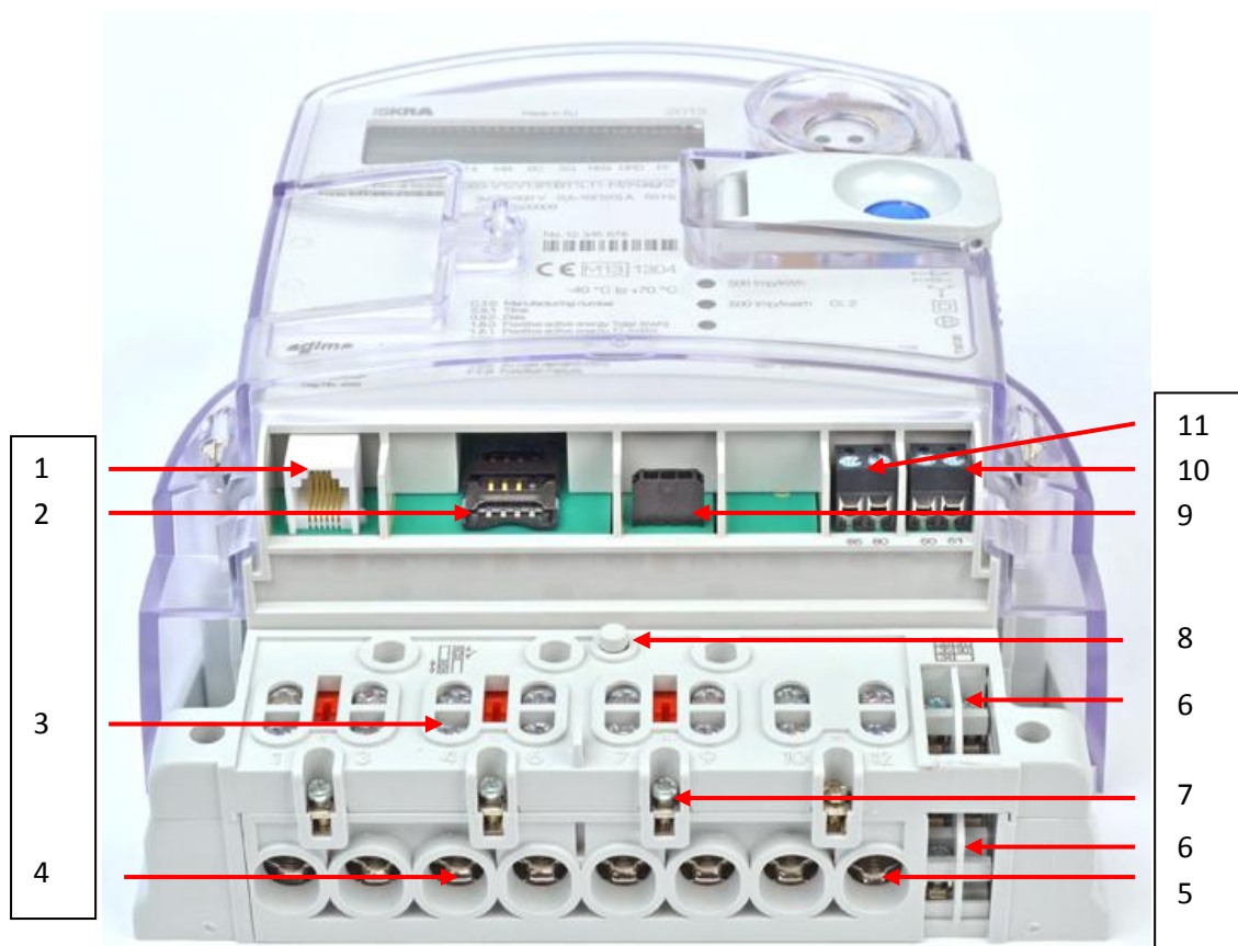
Figure 5: MT382 meter appearance – bottom view
