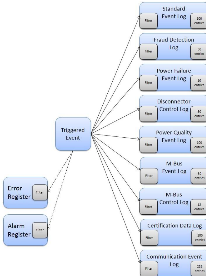
Figure 89: Event handling
