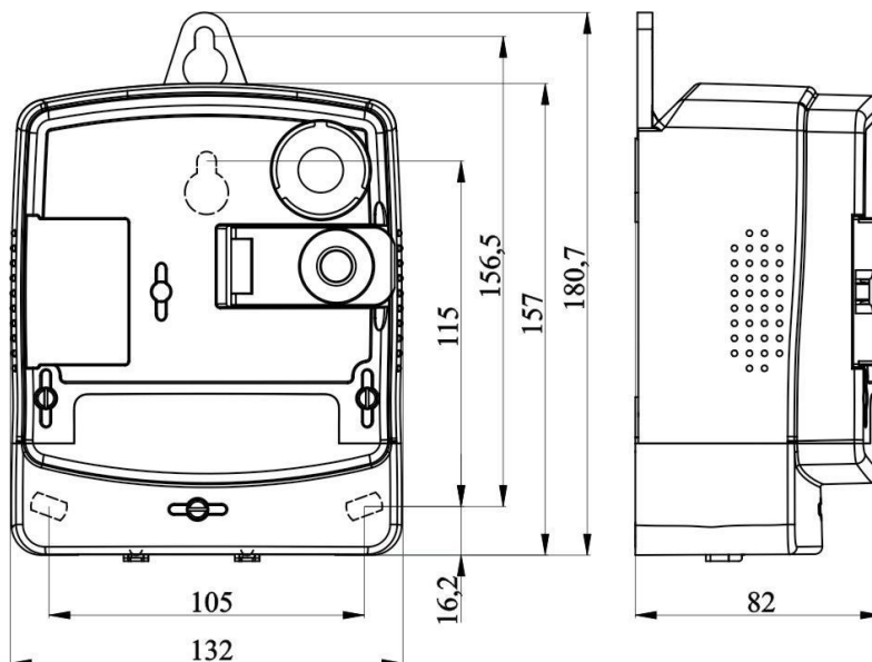
Figure 20: Overall and fixing dimensions of the ME382 meter fitted with a short terminal cover
