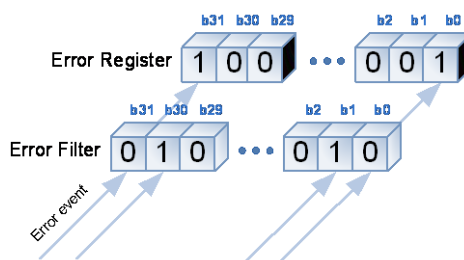
Figure 91: Error filtering
