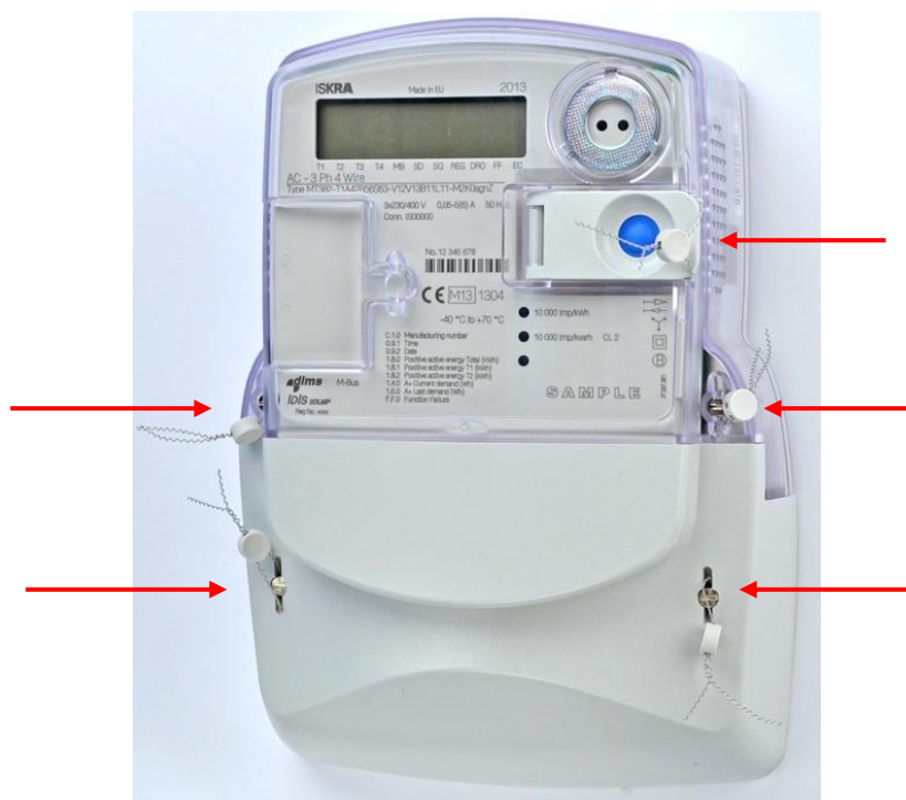
Figure 30: Positions of the seals at MT382 meter
