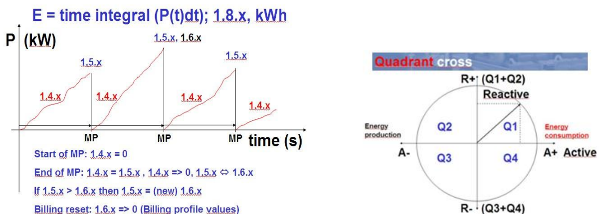
Figure 10: Measuring principle
