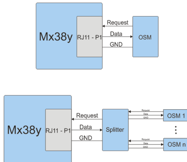
Figure 68: Diagram for connecting device to P1 port
