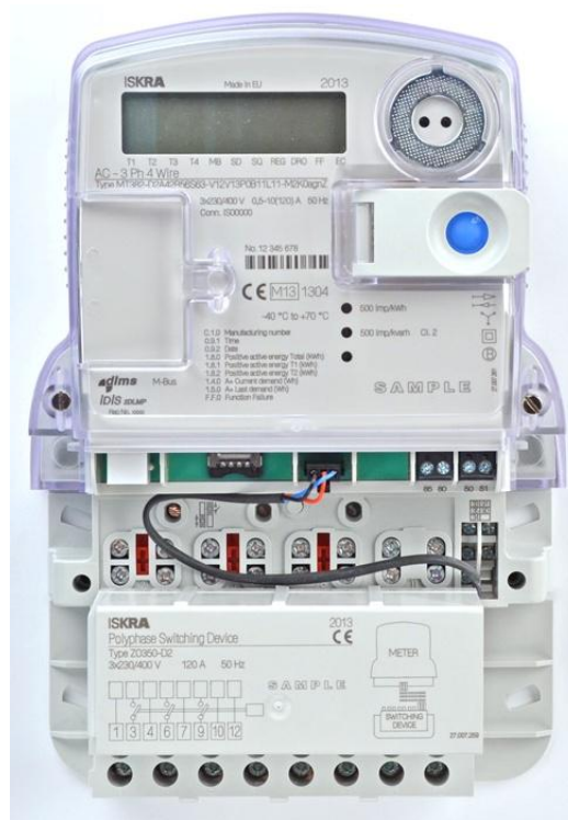
Figure 94: MT382 meter with disconnect
